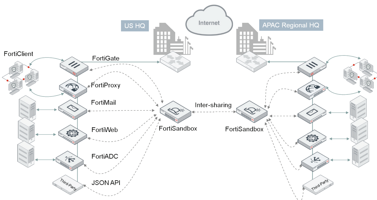
Figure 5: Integrated Deployment
